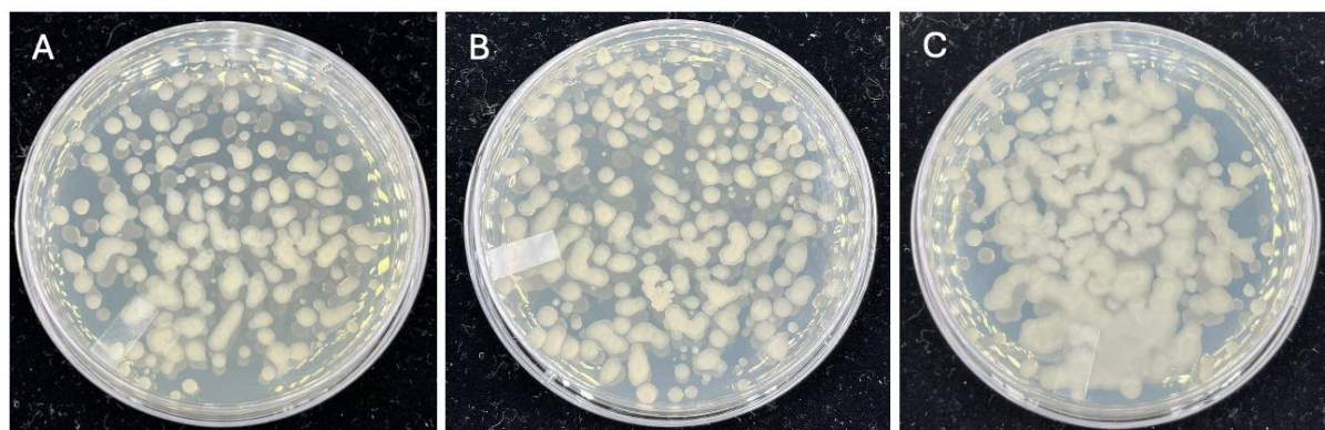
Figure 3. Natural transformation results on LB + Strep 250 plates. A. Bacillus subtilis (SY1483) transformed with Priestia megaterium (SY0032) strep R gDNA. B. Bacillus inaquosorum (SY1167) transformed with Priestia megaterium (SY0032) strep R gDNA. C. Bacillus velezensis (SY1154) transformed with Priestia megaterium (SY0032) strep R gDNA.
