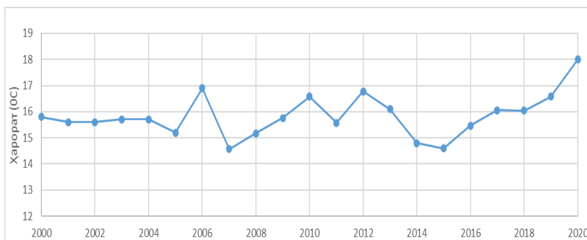
Figure 2. Average long-term temperature graph according to the Bukhara meteorological station
