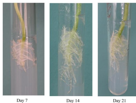
Figure 2. Samples grown in White's test medium with a double dose of potassium nitrate ( \text{KNO}_3 )
