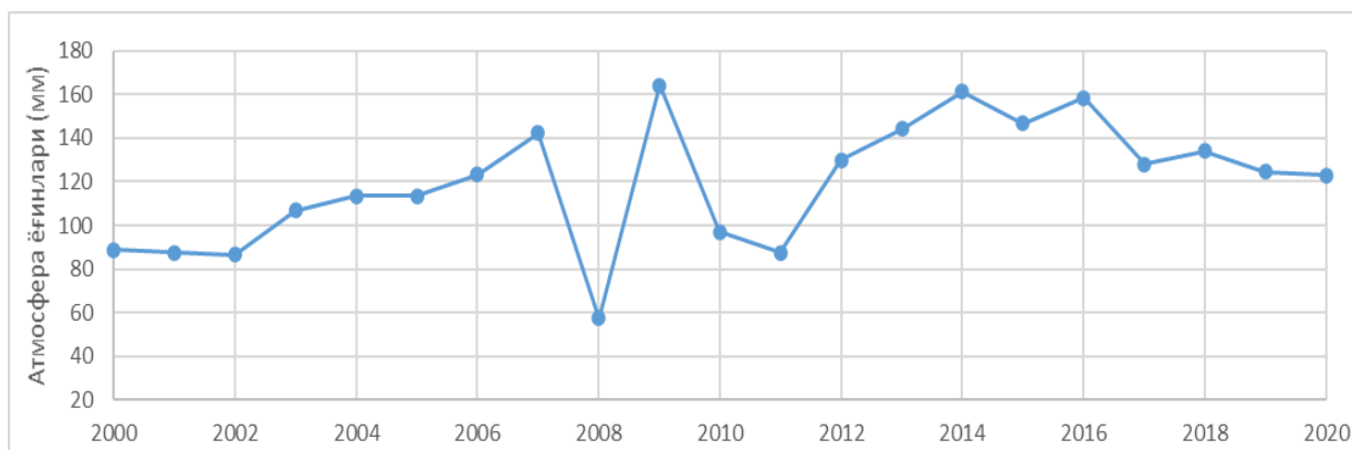
Figure 3. Graph of average long-term atmospheric precipitation according to the Bukhara meteorological station
