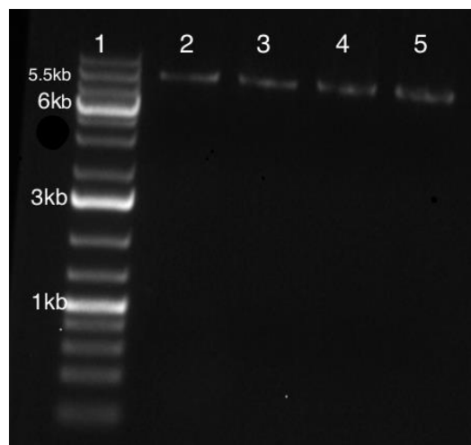
Figure 4. Agarose gel electrophoresis of PepMV plasmid constructs. Lane 1: DNA ladder. Lane 2: pPVP NotI ligated sample. Lane 3: pPVP XhoI ligated sample. Lane 4: pPVP NotI unligated control. Lane 5: pPVP XhoI unligated control.
