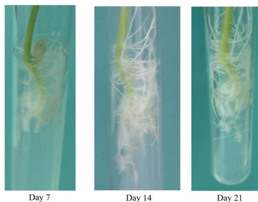
Figure 3. Samples grown in White's test medium with a double dose of calcium nitrate ( \text{Ca}(\text{NO}_3)_2 )
