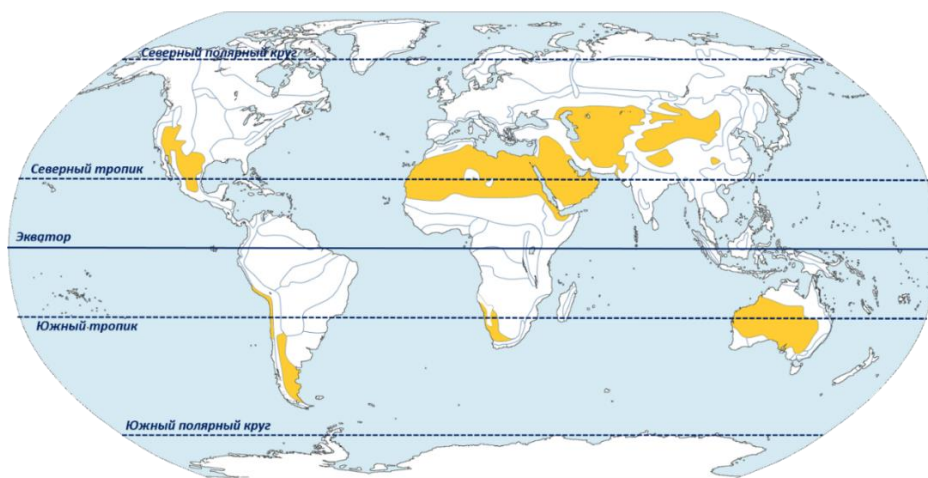
Figure 4. Location of arid regions on the Earth's surface
