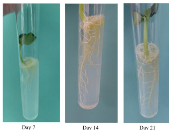
Figure 1. Samples grown in White's control medium
